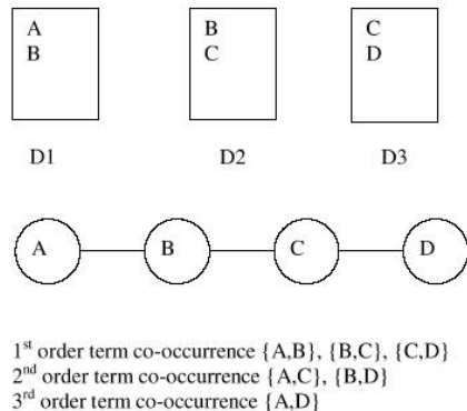
Fig. 1. Higher-order co-occurrences [5]
